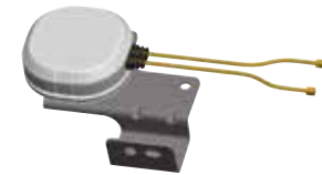
(GPS / GSM) GPS354P-S3-12-A 60x60x15 mm
