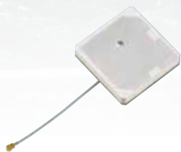
B3G02N-S3-01-A 49.14x46.14x15.94mm
